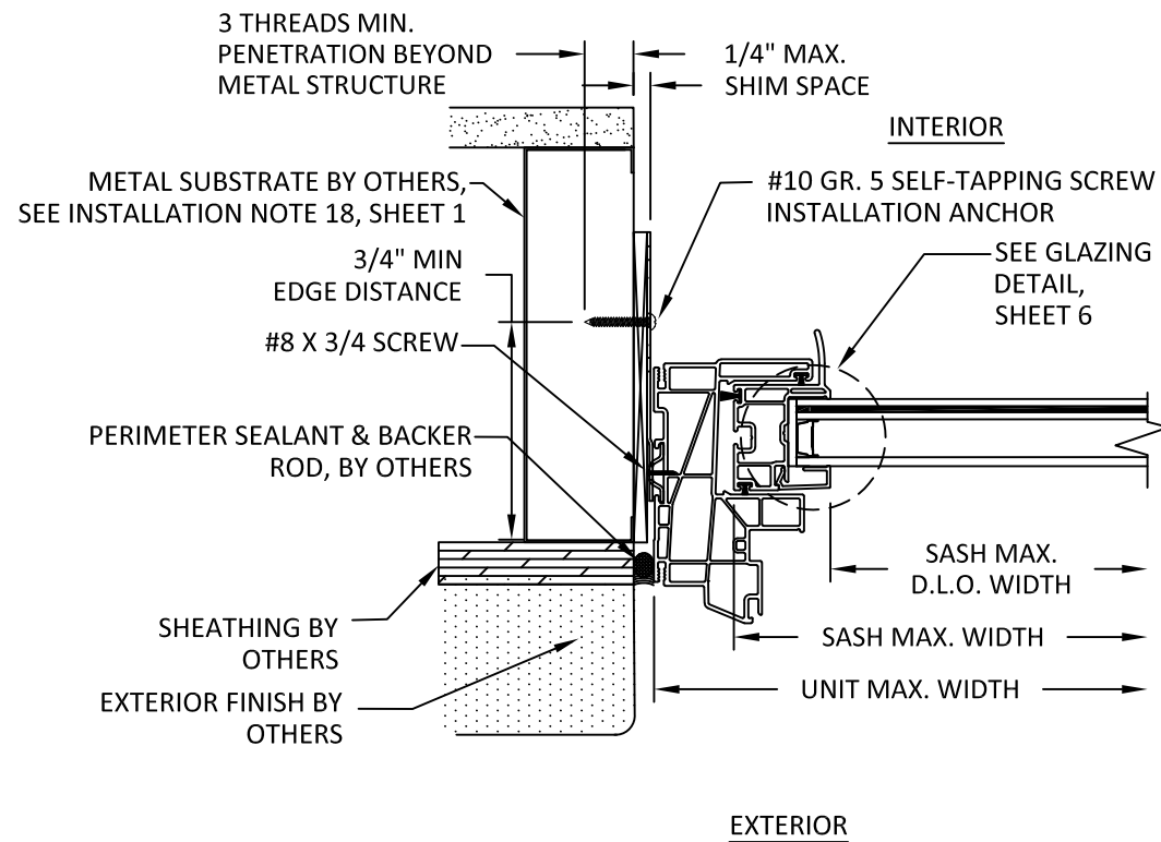
B 5 HORIZONTAL SECTION CLIP INSTALLATION METAL STUD
